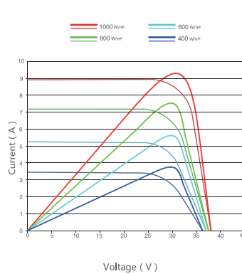
Current-Voltage & Power-Voltage Curves (260W)
